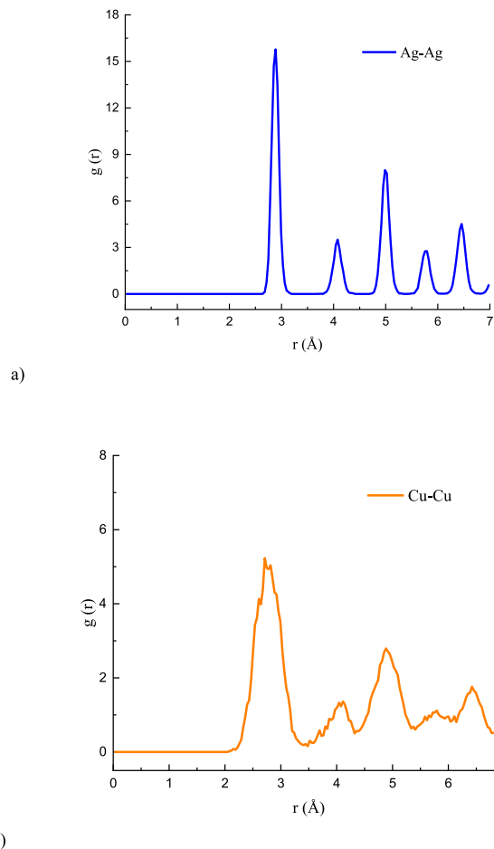
Fig. 6. The RDF output of a) Ag and b) Cu samples after equilibrium phase detection inside the computational box.
